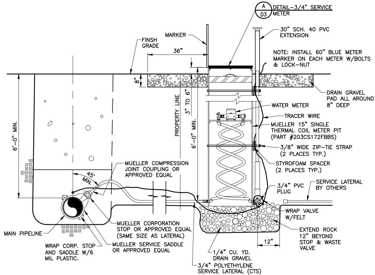
A TYP DETAIL-WATER SERVICE CONNECTION ASSEMBLY NO SCALE
